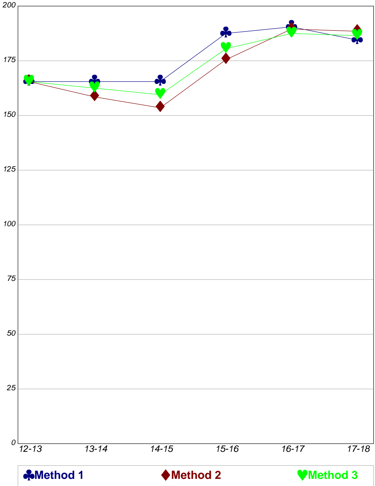
Graph 14 6-8 Enrollment 2012-2017 Comparison between projection methods
